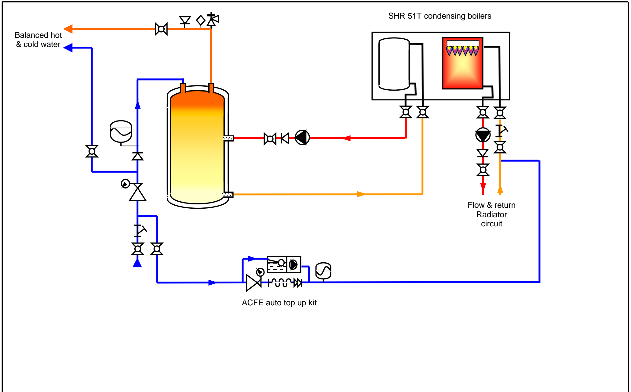
Typical pipework arrangement combi boiler
