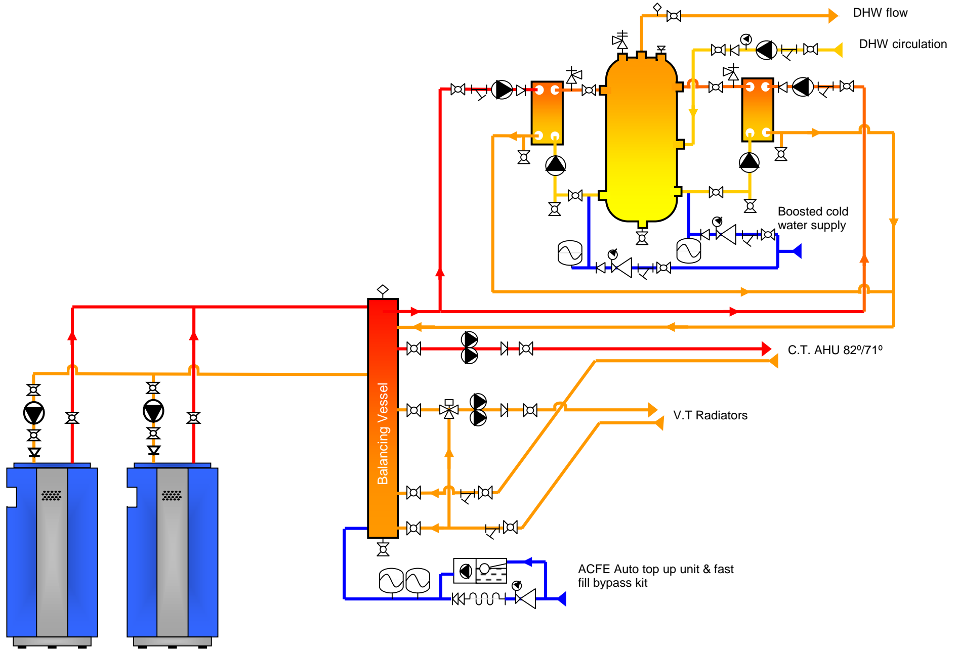
Mutliple boiler pipework arrangement generating DHW through an expresso packaged plate heat exchanger with buffer storage
